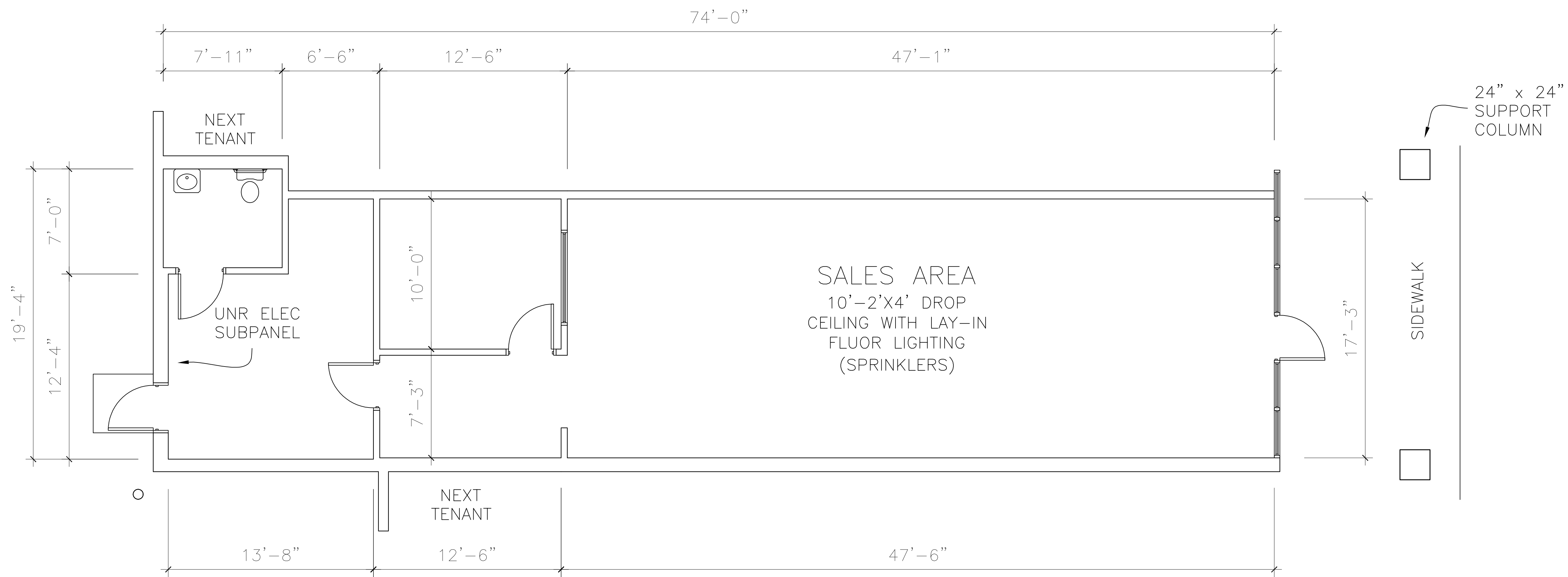
EXISTING FLOOR PLAN: SCALE: 1/4" = 1'
