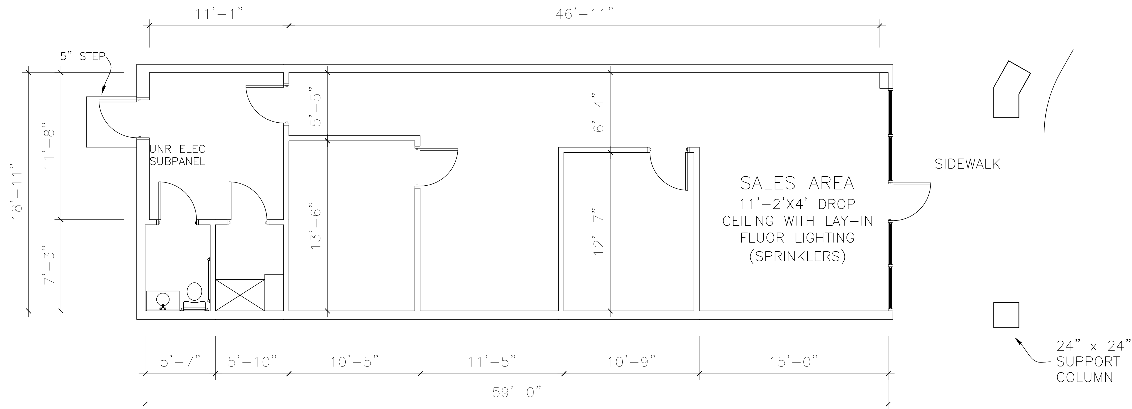
EXISTING FLOOR PLAN: SCALE: 1/4" = 1'
