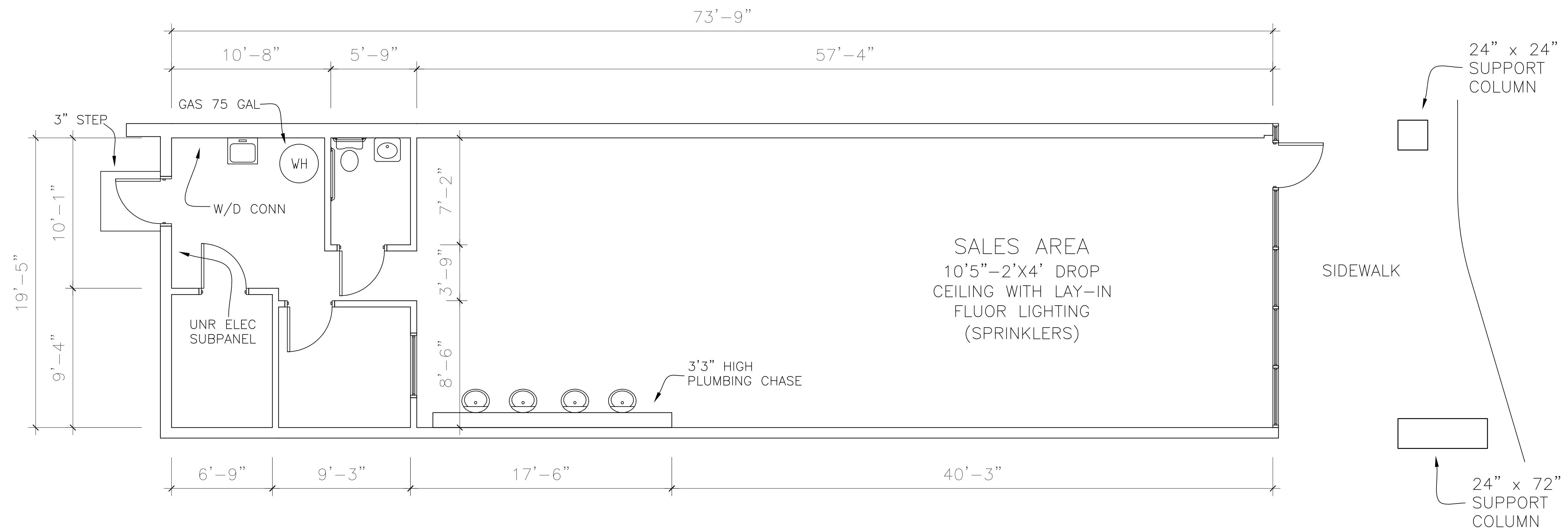
EXISTING FLOOR PLAN: SCALE: 1/4" = 1'
