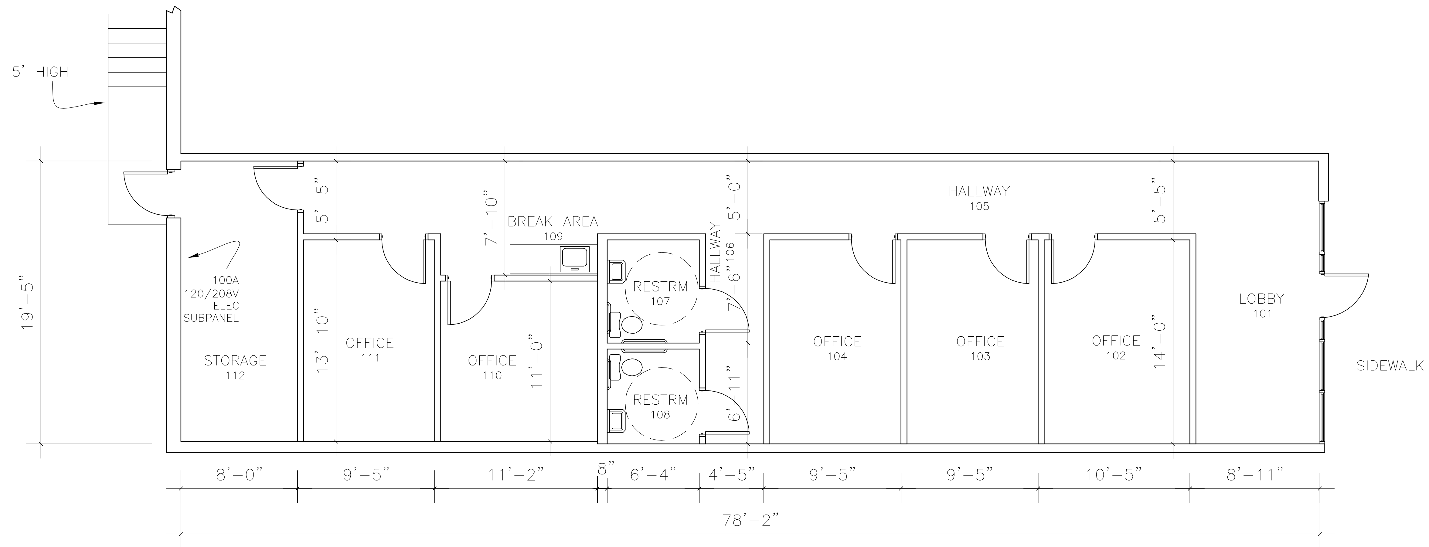
EXISTING FLOOR PLAN: SCALE: 1/4" = 1'
