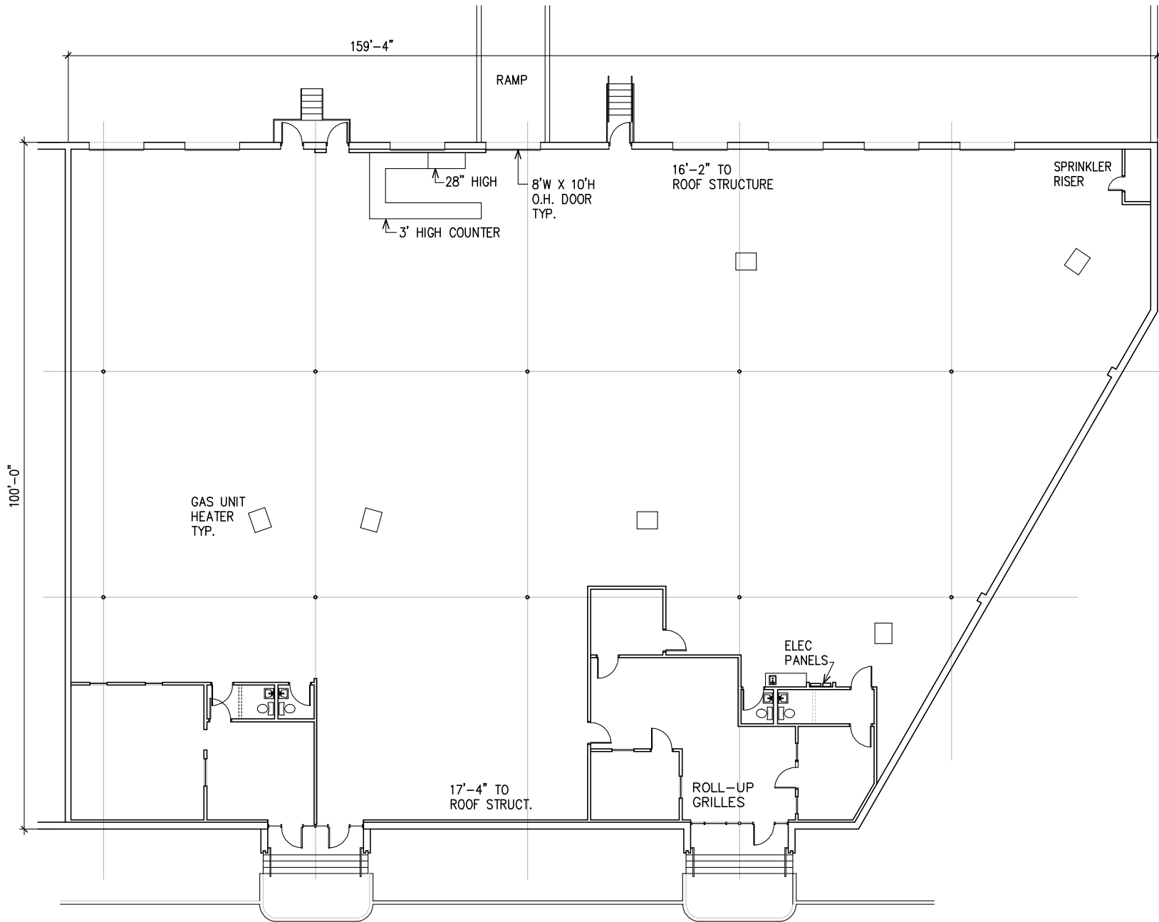
FLOOR PLAN
