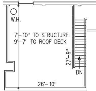
MEZZANINE PLAN
