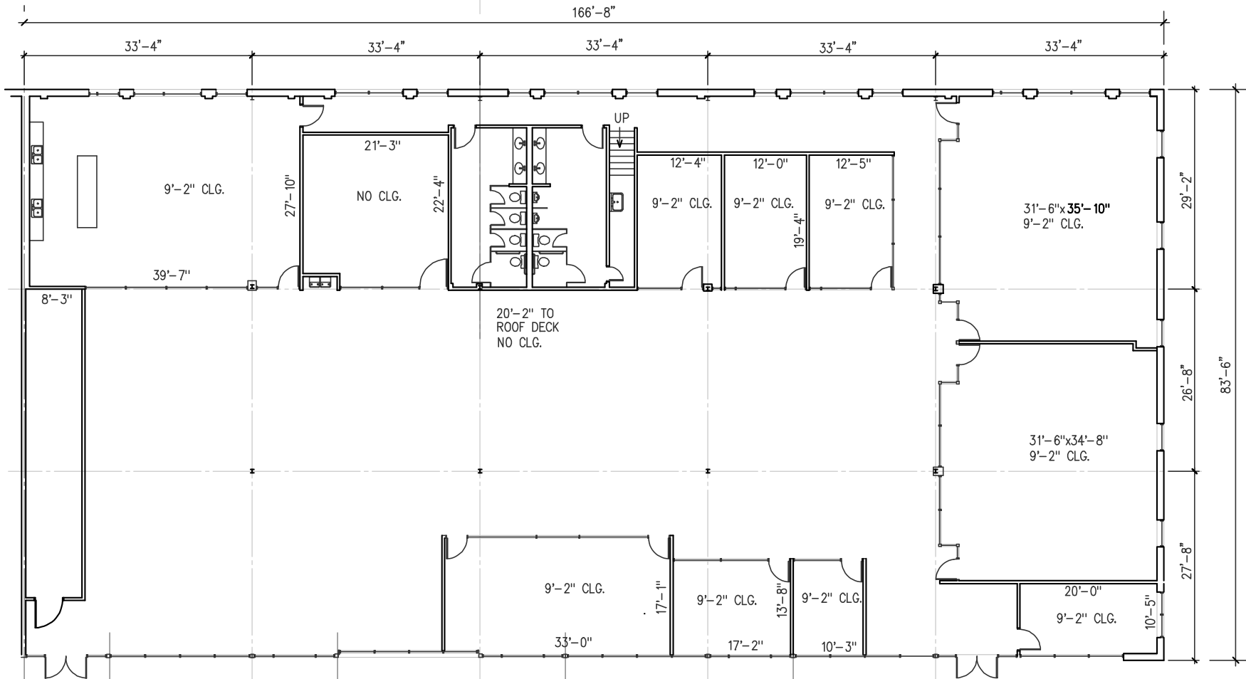
FLOOR PLAN
