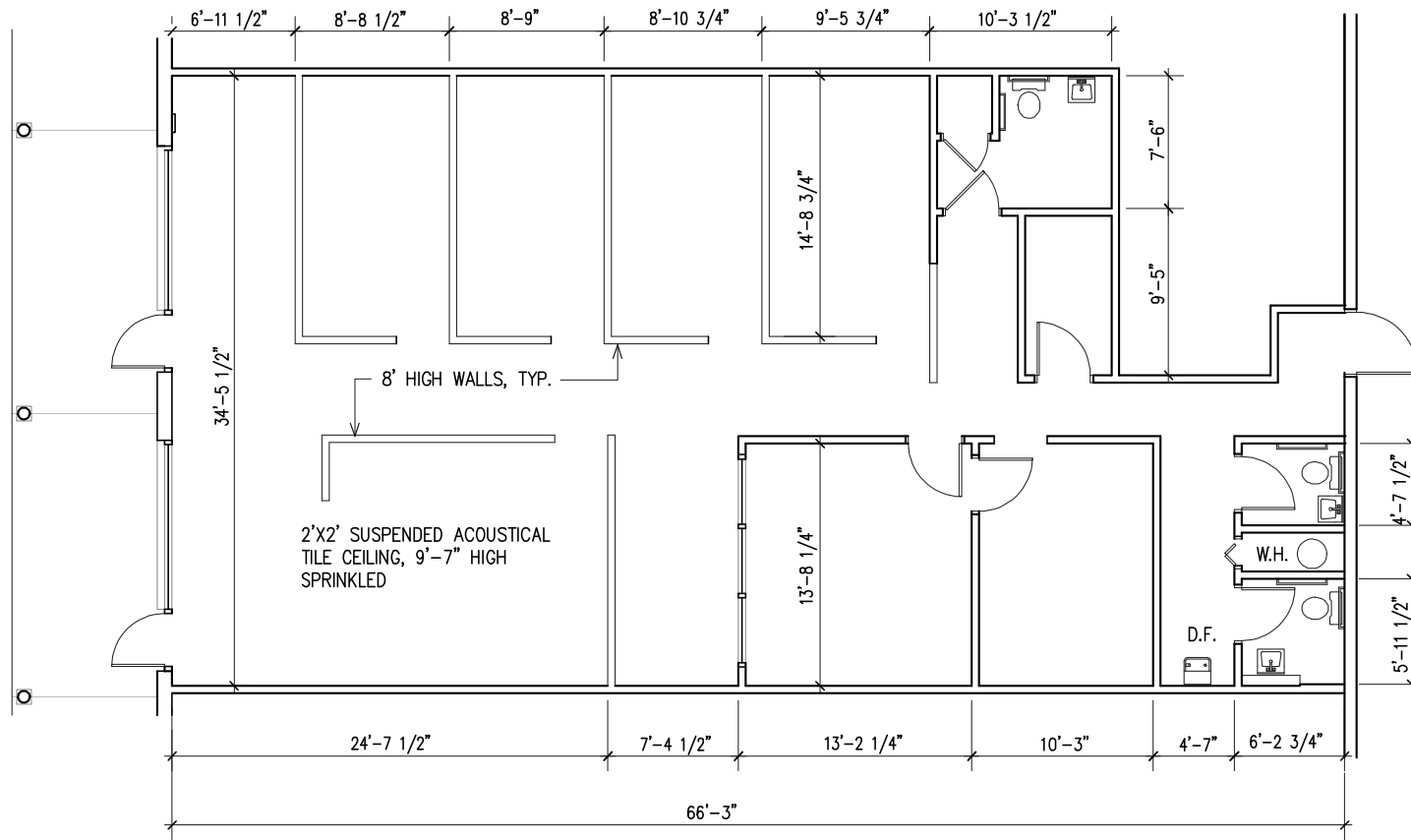
FLOOR PLAN
