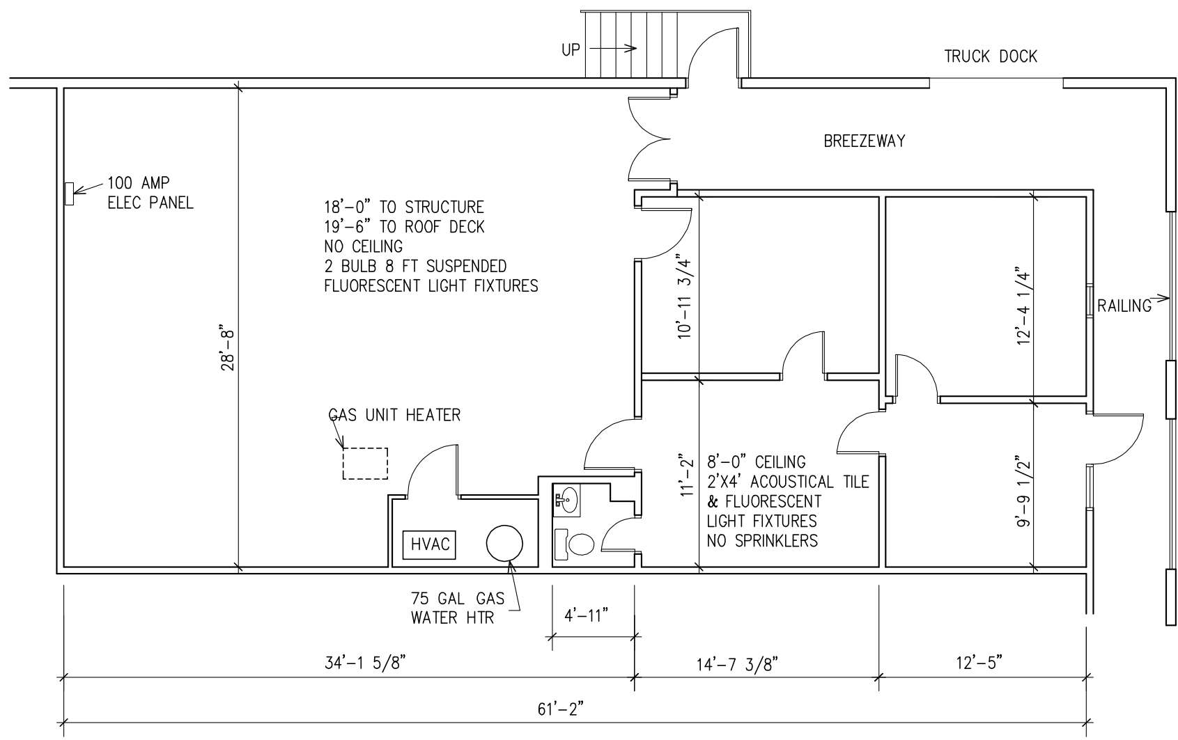
FLOOR PLAN
