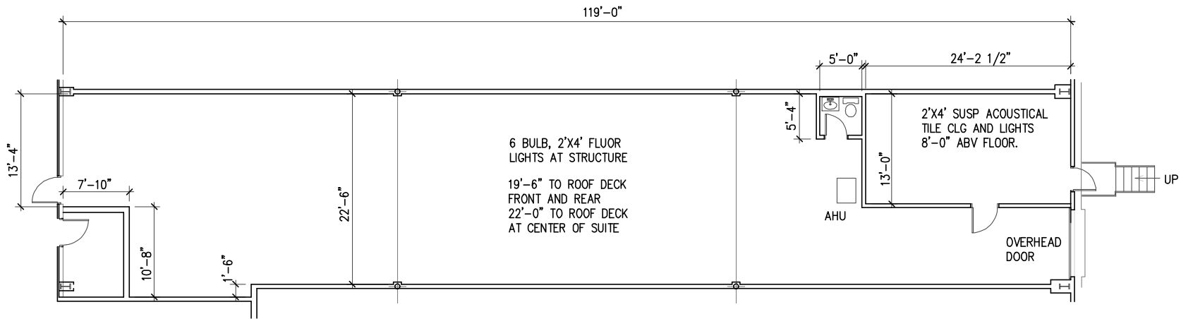
FLOOR PLAN SUITE E
