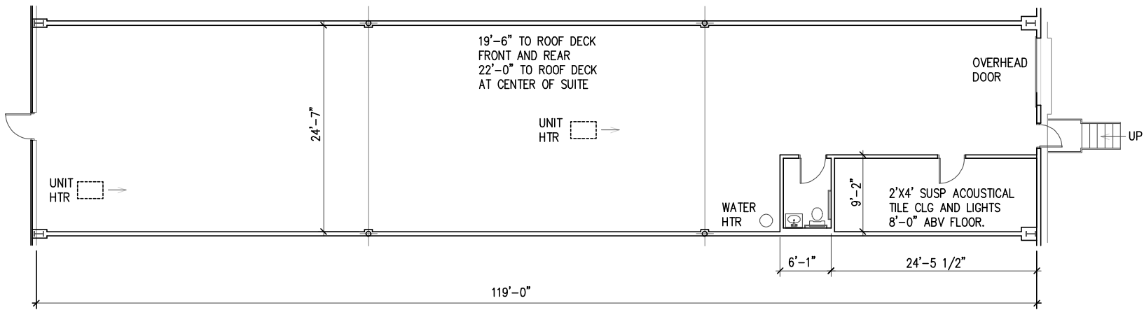
FLOOR PLAN SUITE D 0' 4' 8' 12' 16' 20'
