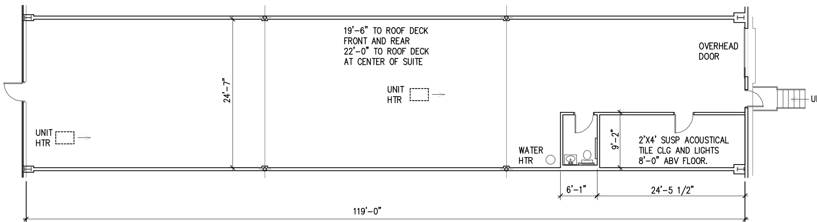
FLOOR PLAN SUITE D
