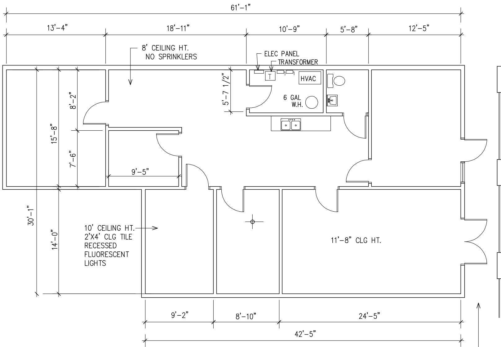
FLOOR PLAN
