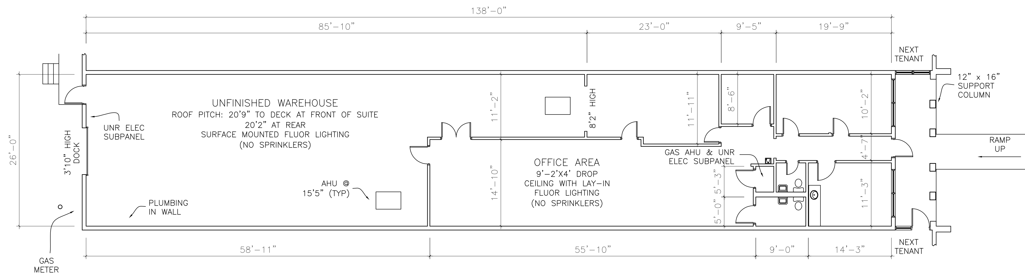
EXISTING FLOOR PLAN: SCALE: 1/8" = 1'
