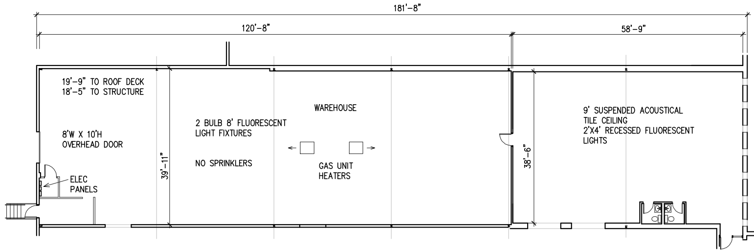
FLOOR PLAN
